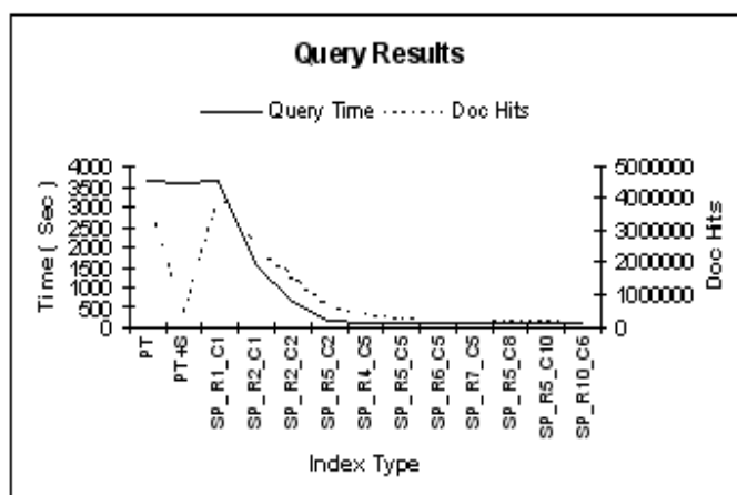
Fig. 5. Query results.
