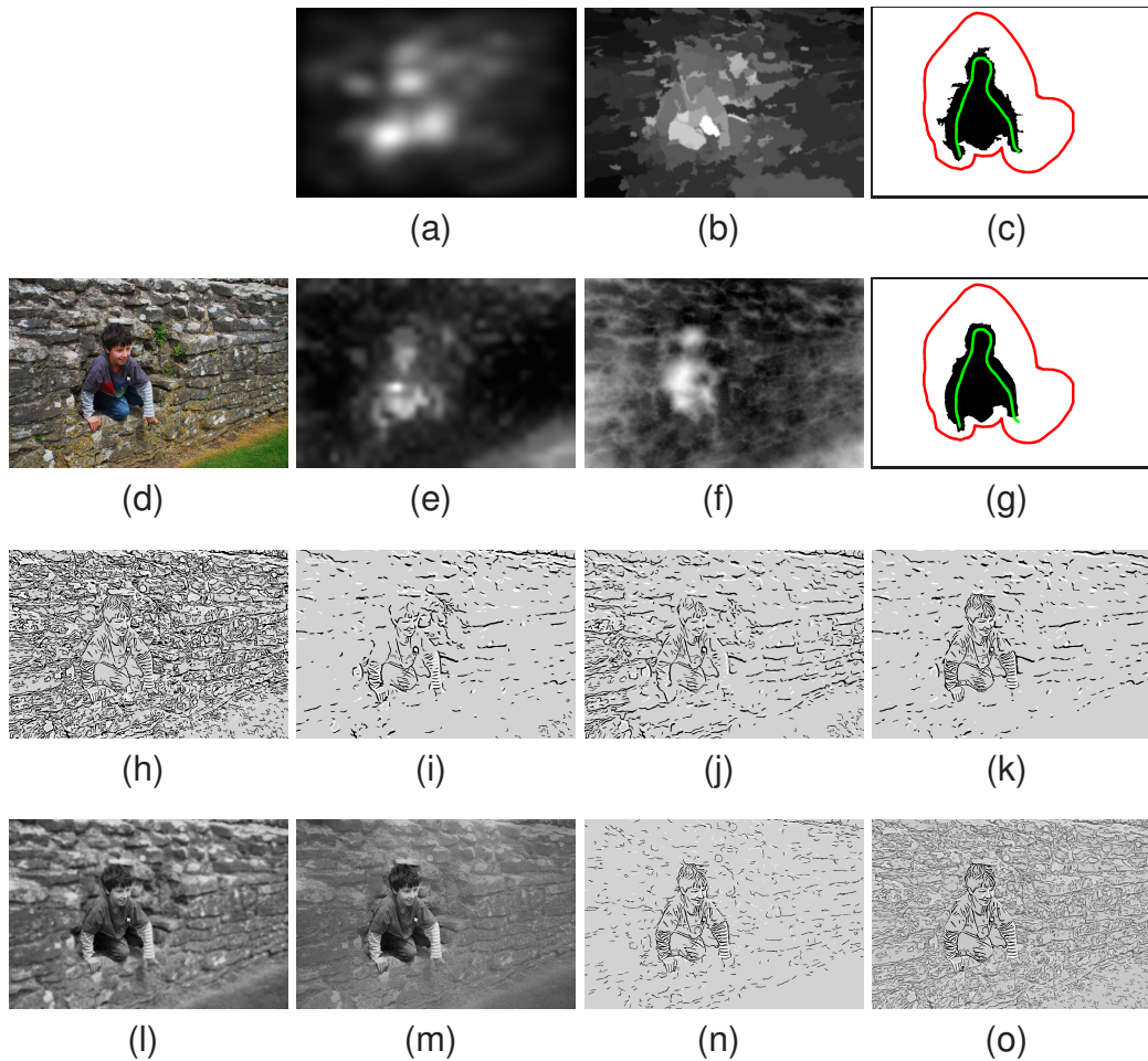
Fig. 11. Incorporating saliency to modify level of detail: d) original image, a) saliency map using method by [41], b) saliency map using method by [40], e) saliency map using method by [42], f) saliency map using method by [43], c) mask showing initial scribbles for foreground and background after supervised watershed segmentation [38], g) mask after refinement with Grabcut [33], h) our basic three tone rendering, i) three tone rendering after image is blurred using saliency map from [42], j) three tone rendering after image is blurred using saliency map from [43], k) three tone rendering after image is blurred using foreground mask, l) image blurred using foreground mask, m) background contrast reduced using Poisson reconstruction, n) three tone rendering from Poisson reconstruction, o) background lines from our basic three tone rendering rescaled (giving five tones).
