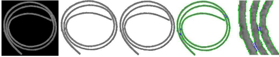
Figure 15: From left to right: original slice; segmentation by Graph Cut with the shape prior; final result after postprocessing to separate layers; postprocessed slice and contour of its neighbour slice (shown in green, with blue marks indicating postprocessing areas); close-up
