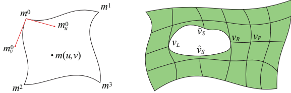
Figure 2: Ferguson patch and topology-preserving gradient mesh.
