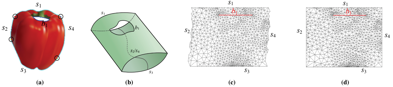
Figure 6: Topology-related mapping for an image region with a hole: (a) input image region with hole, (b) corresponding topological cylinder with hole, (c) quasi-rectangle in the parameter domain, with slit, (d) corrected rectangle with slit in the parameter domain. The triangulations in (c) and (d) have been reduced to make them clearer.
